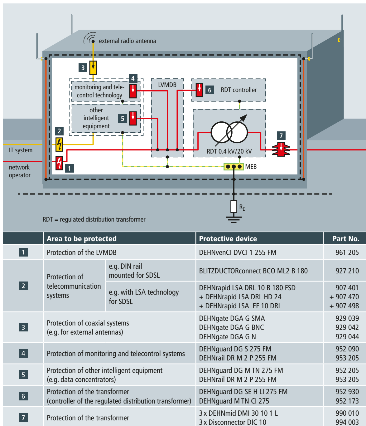
Figure 4 Example of lightning and surge protection measures for an intelligent transformer substation
