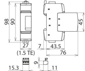
Dimension drawing DG SE H LI 275 FM
