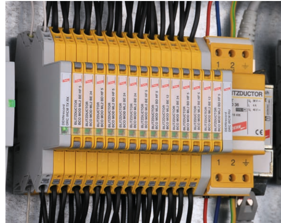
Figure 12 BLITZDUCTOR: combined arrester with actiVsense technology and integrated LifeCheck monitoring
